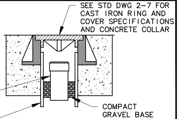
CLEAN OUT DETAIL FOR HARDSCAPE AREAS
