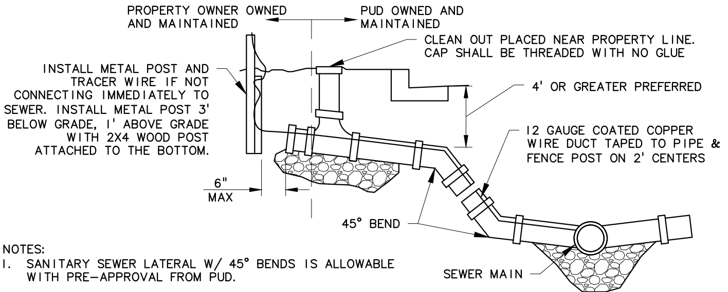
CLEAN OUT DETAIL FOR LANDSCAPE AREAS
