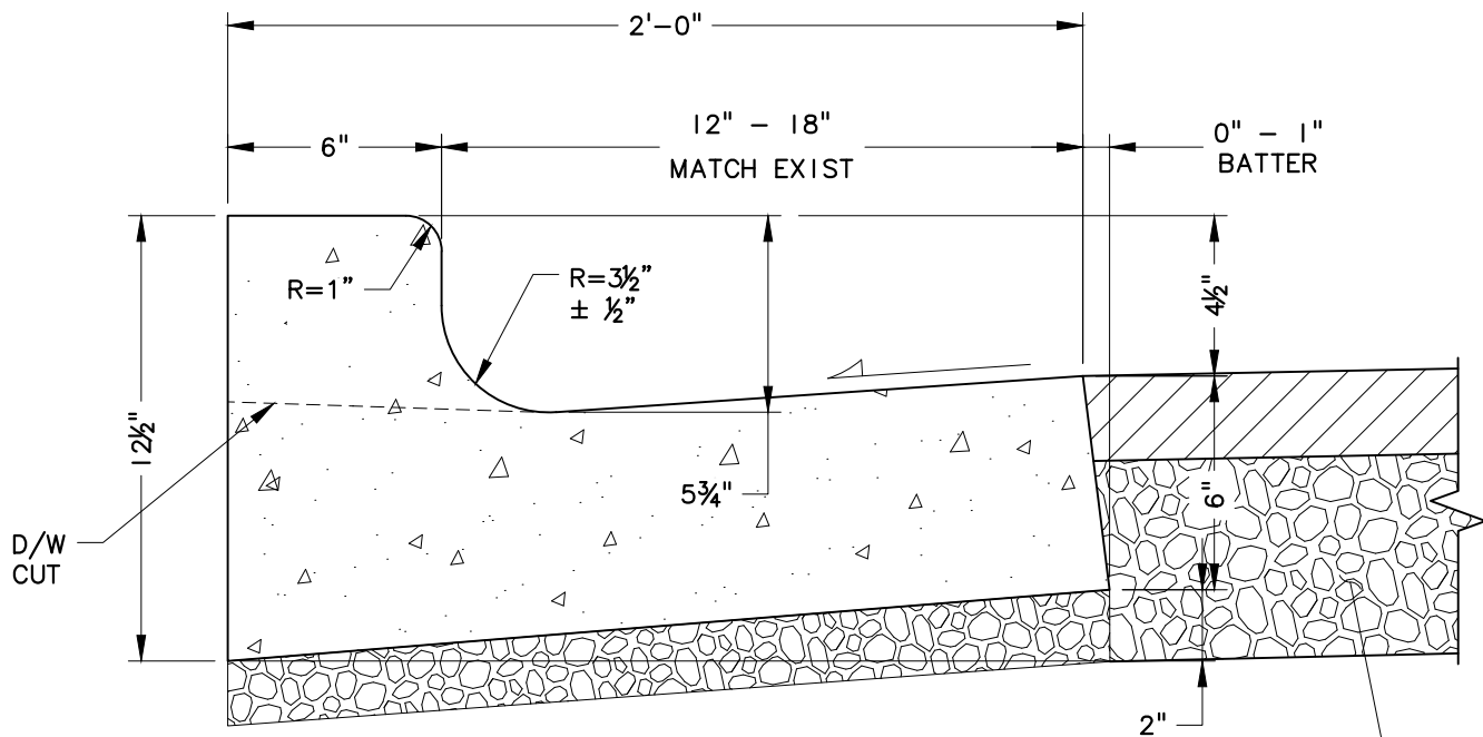
CONCRETE CURB AND GUTTER
