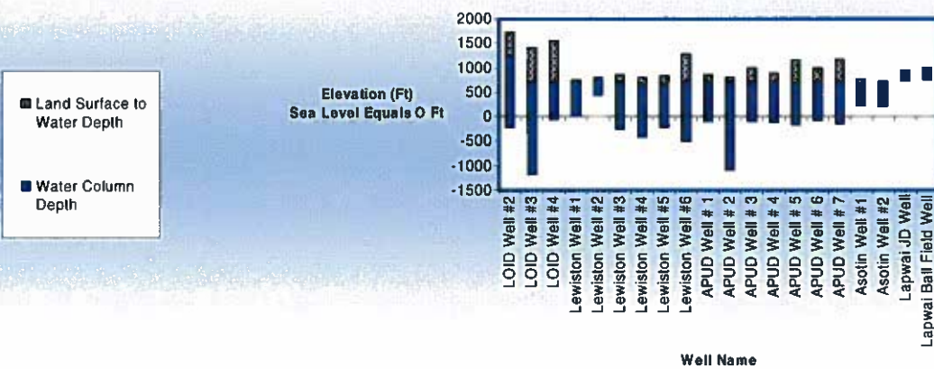
Lewis Clark Valley Municipal Well Profiles Chart
