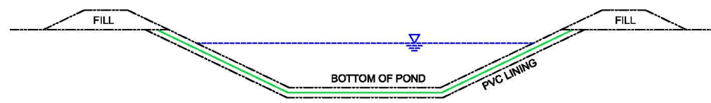
PVC LINED POND
