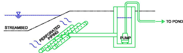
INFILTRATION TO PUMP
