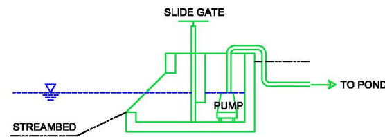
DIRECT PUMP
