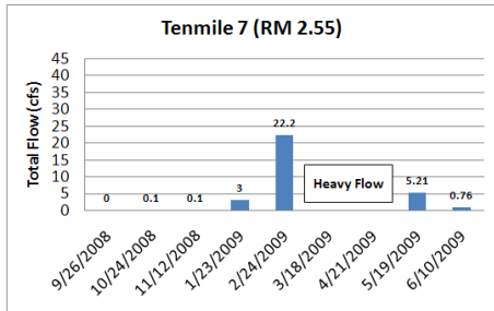
Figure C.8. Study streamflow data for Tenmile Creek.
