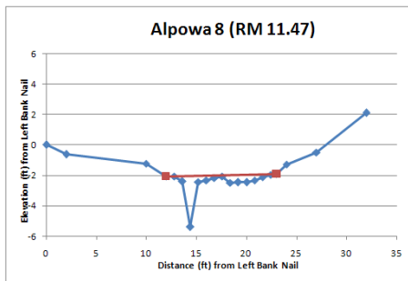
Figure B.2. Transect plots for Alpowa Creek with water level at time of measurements shown by red line.
