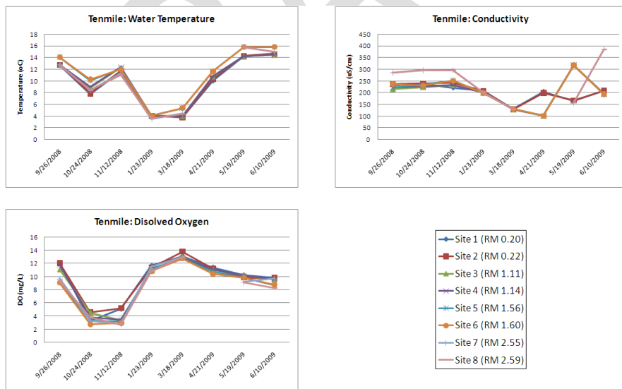
Figure G.11. Water temperature, dissolved oxygen and conductivity data for Tenmile Creek.
