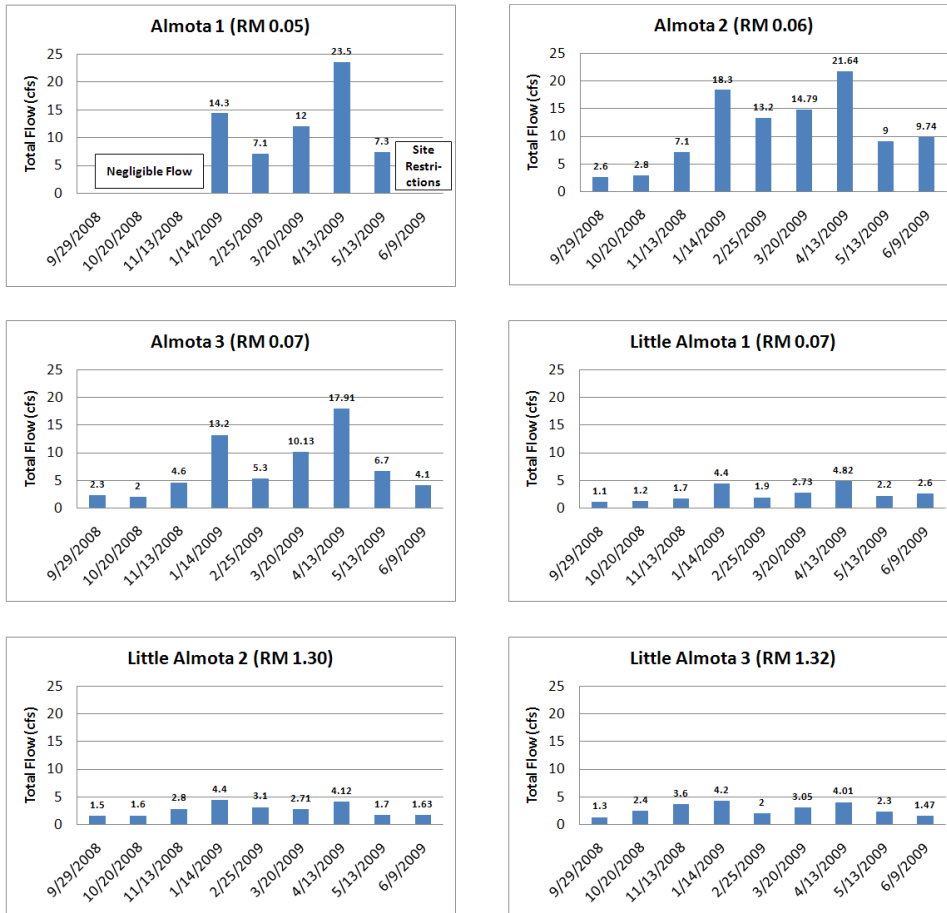
Figure C.1. Study streamflow data for Almota and Little Almota Creeks.
