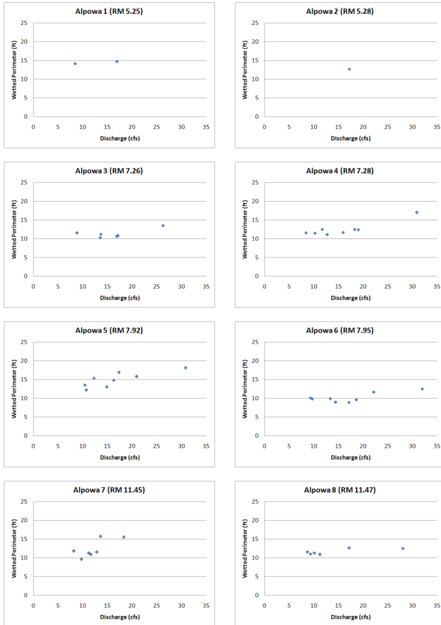
Figure E.2. Wetted perimeter versus discharge plots for Alpowas Creek.
