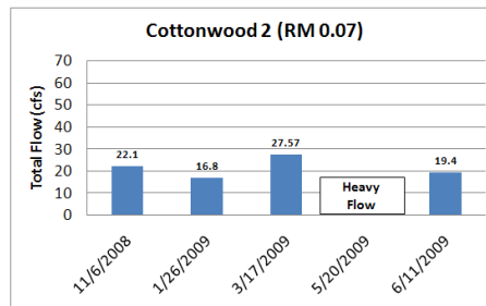
Figure C.6. Study streamflow data for Joseph and Cottonwood Creeks.
