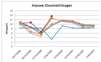
Figure G.4. Water temperature, dissolved oxygen and conductivity data for Alpowa Creek.
