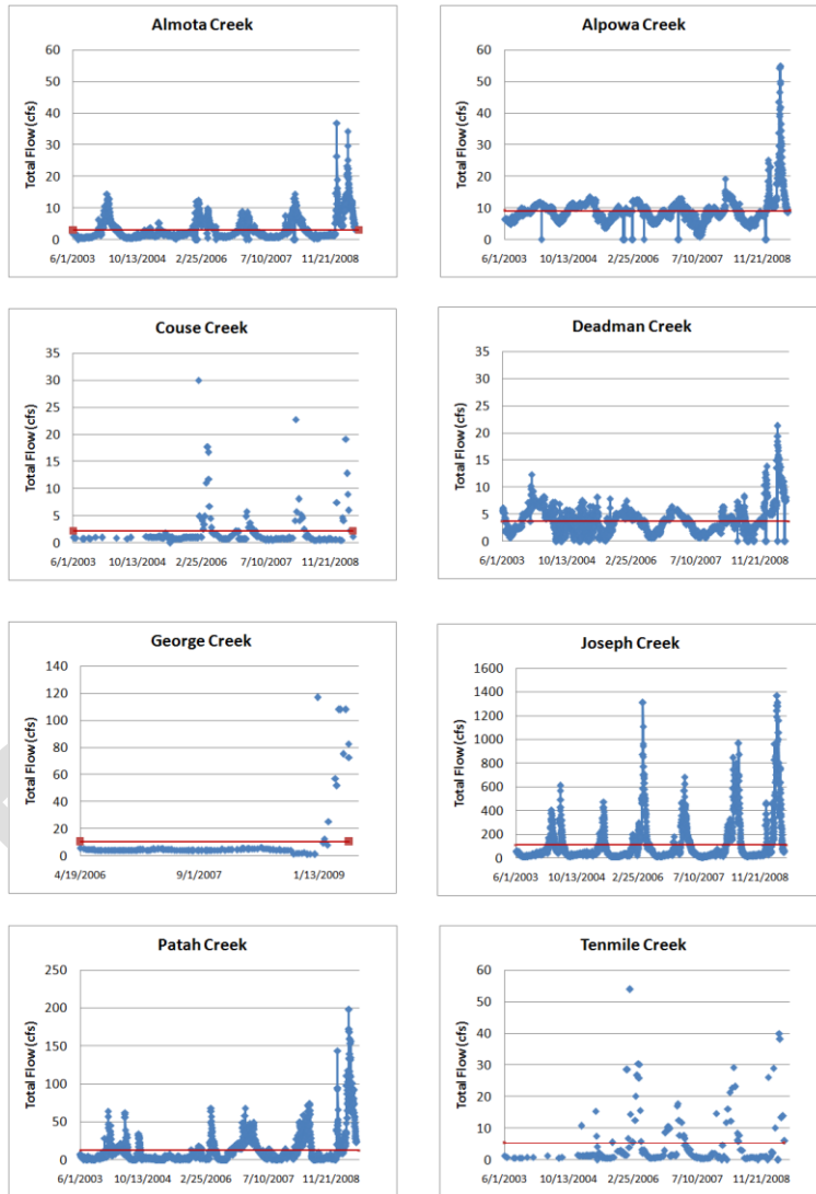
Figure D.1. Streamflow data collected by Washington State Department of Ecology for WRIA 35 streams. The red line represents the average flow over the 2003-2009 period for which data is available.
