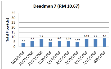
Figure C.4. Study streamflow data for Deadman Creek.
